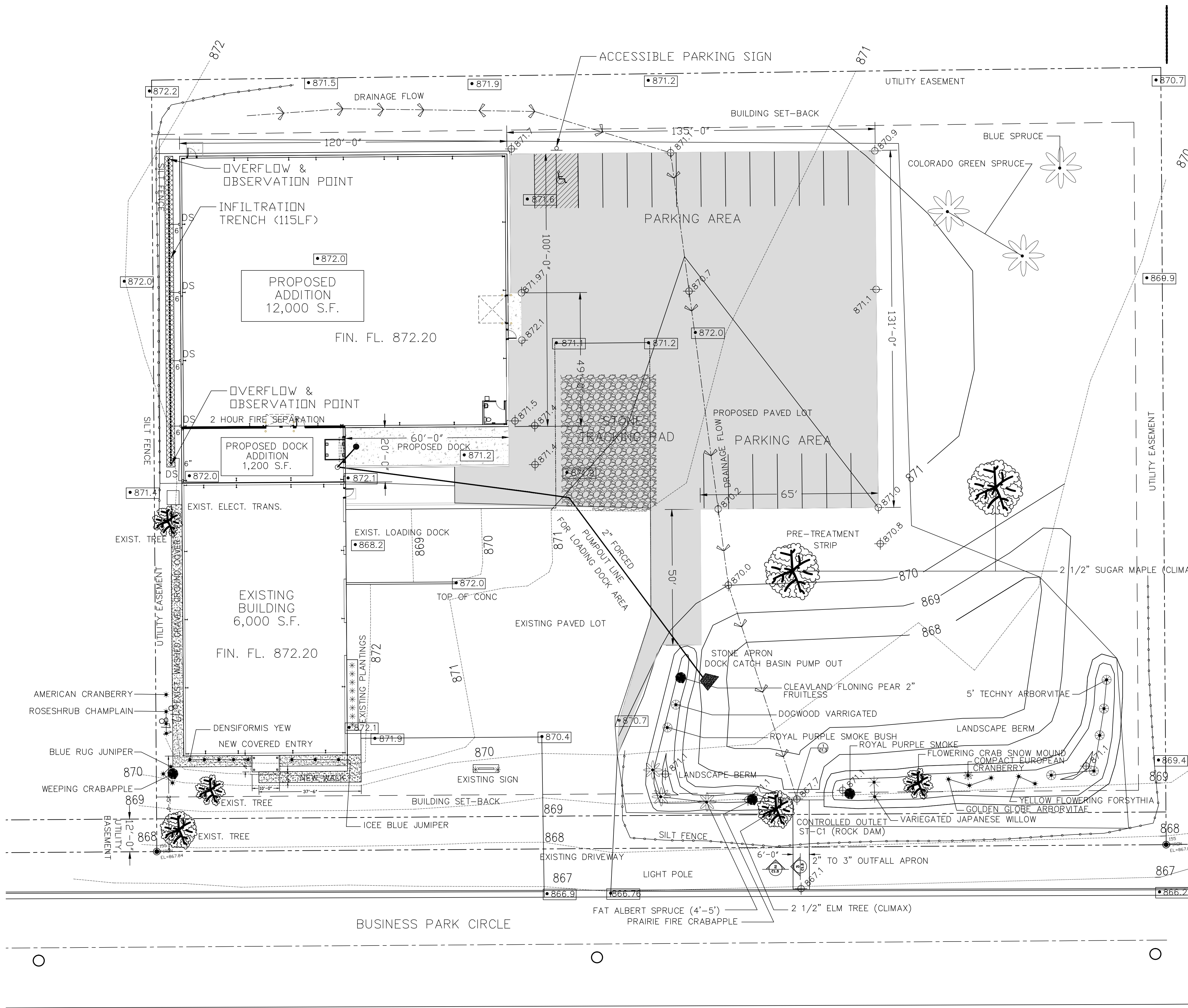
LANDSCAPE PLAN SCALE: 1" = 20'
